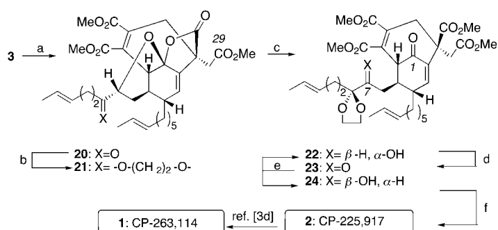
Scheme 5. a) TMSCHN 2 , 15 min, >90%; b) (TMSOCH 2 ) 2 , TMSOTf, CH 2 Cl 2 , 5 h, 90%; [6] c) 1. LiOH, THF/H 2 O, 1.2 h; 2. TMSCHN 2 , 0.5 h, 70% overall; d) Dess–Martin periodinane, NaHCO 3 , CH 2 Cl 2 , 4 h, 90%; e) LiAlH(O t Bu) 3 , toluene, –10°C, 5 min, 70%, 22:24 = 1:1; f) 1. LiOH, THF–H 2 O, 24 h; 2. TFA/CH 2 Cl 2 /H 2 O (54/4/1), 30 min, 70% overall.
